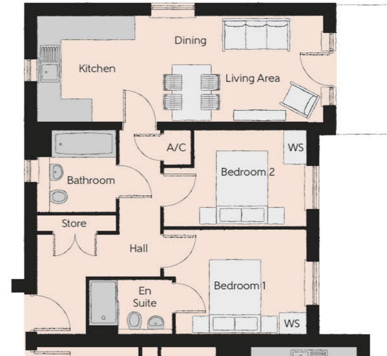
Plots 72 & 75 (First floor shown)
